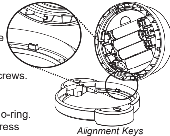
Alignment Keys
