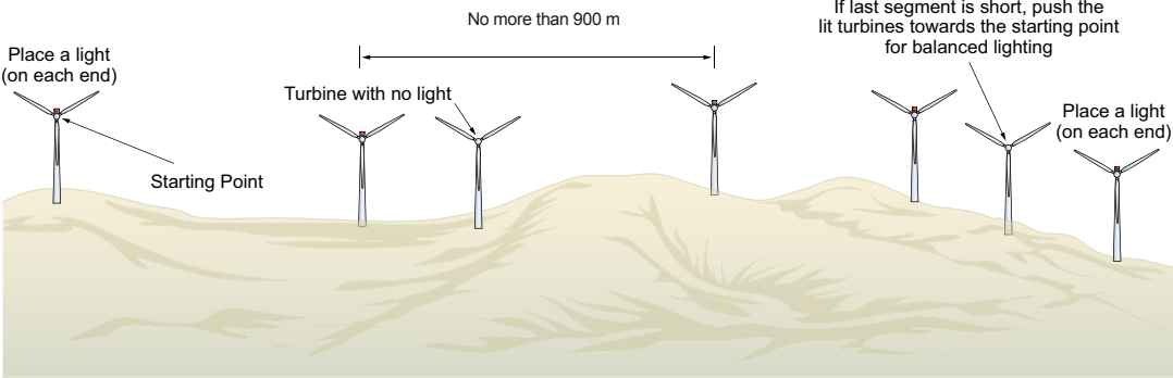
Linear Turbine Configuration
